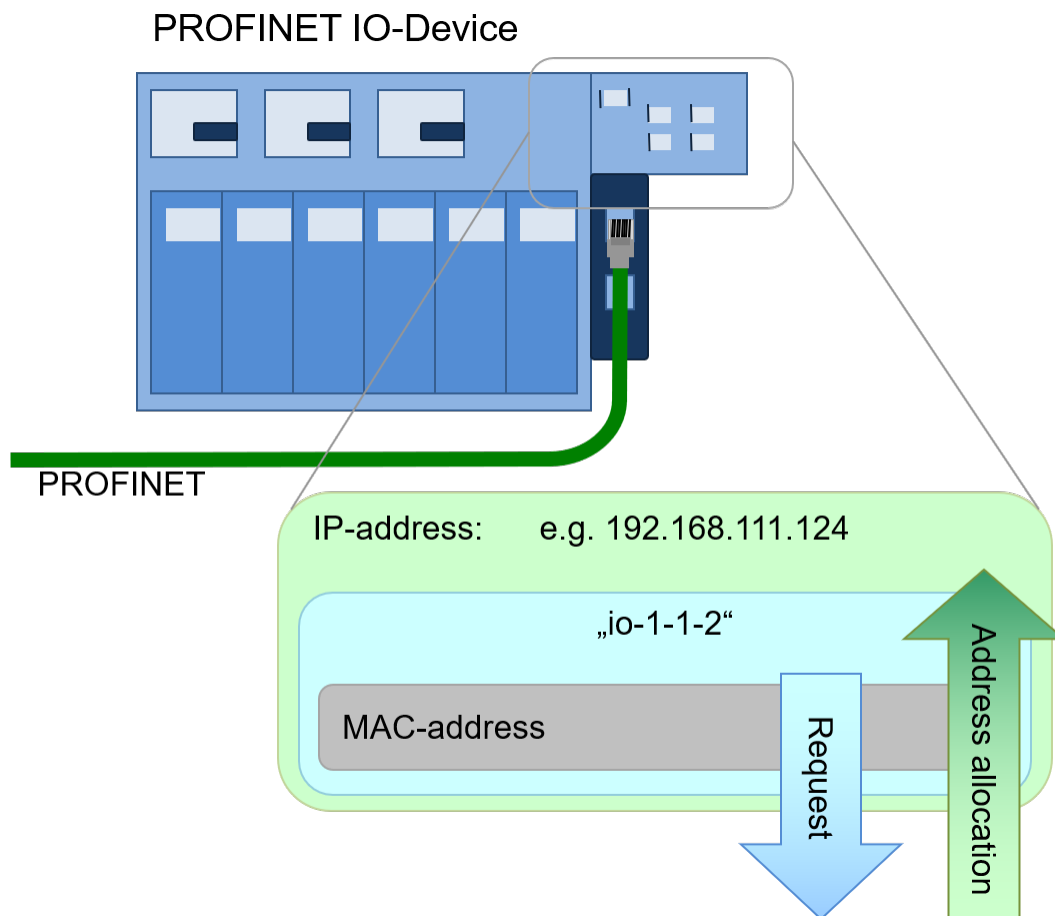
Figure 7-2: PROFINET IO device (address allocation)
