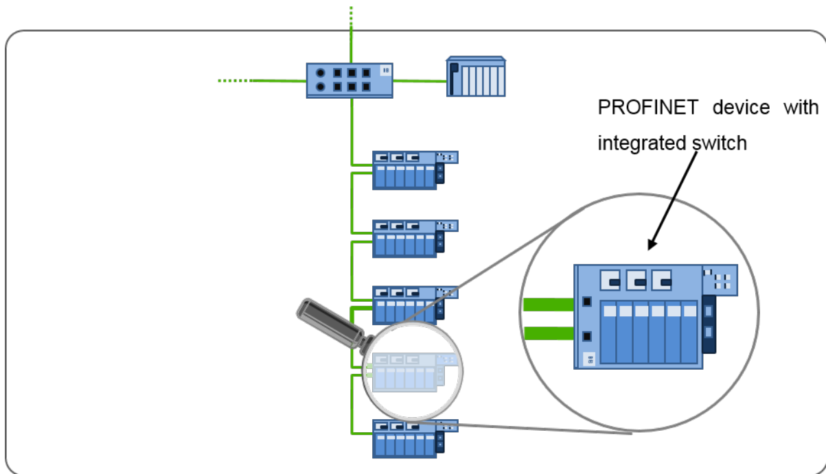
Figure 3-3: Line topology
