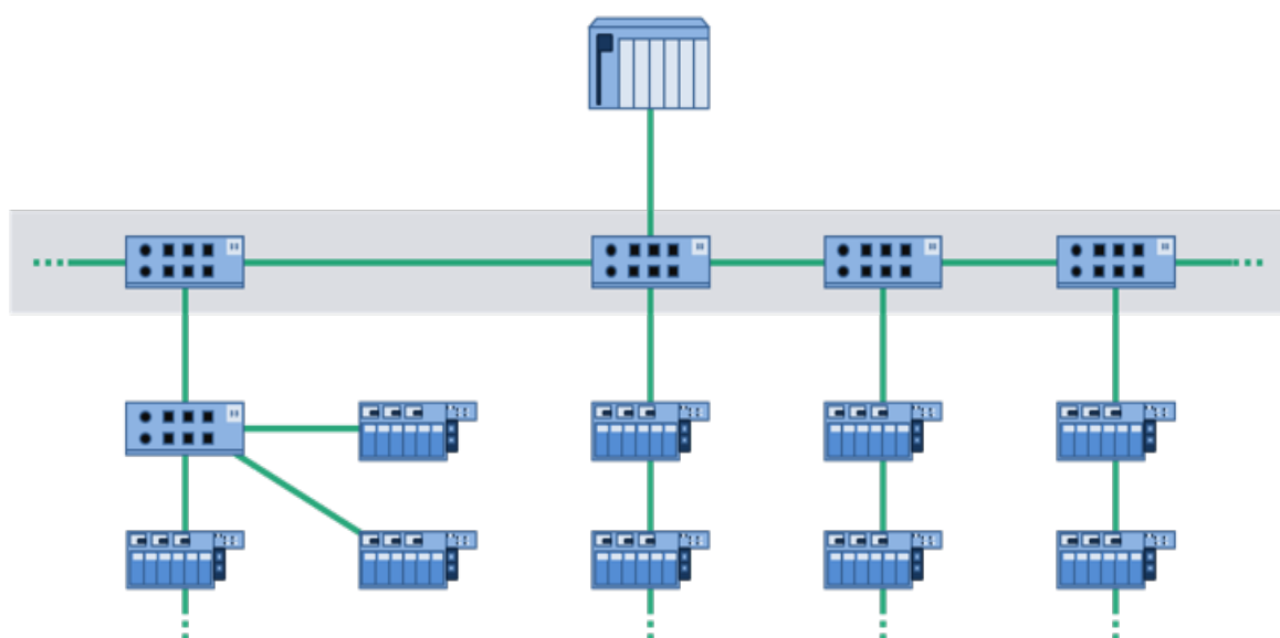
Figure 3-5: Topology example
