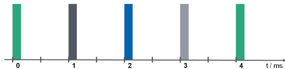
Figure 5-3: Network load, transmission cycle 4 ms, controller transmission clock 1 ms
