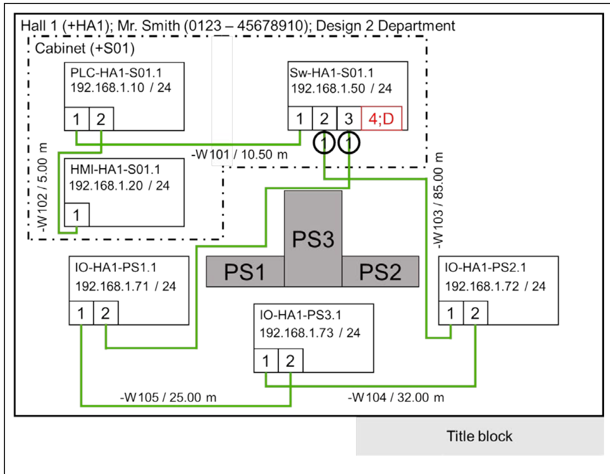
Figure 9-29: Example of PROFINET forwards documentation, ring topology
