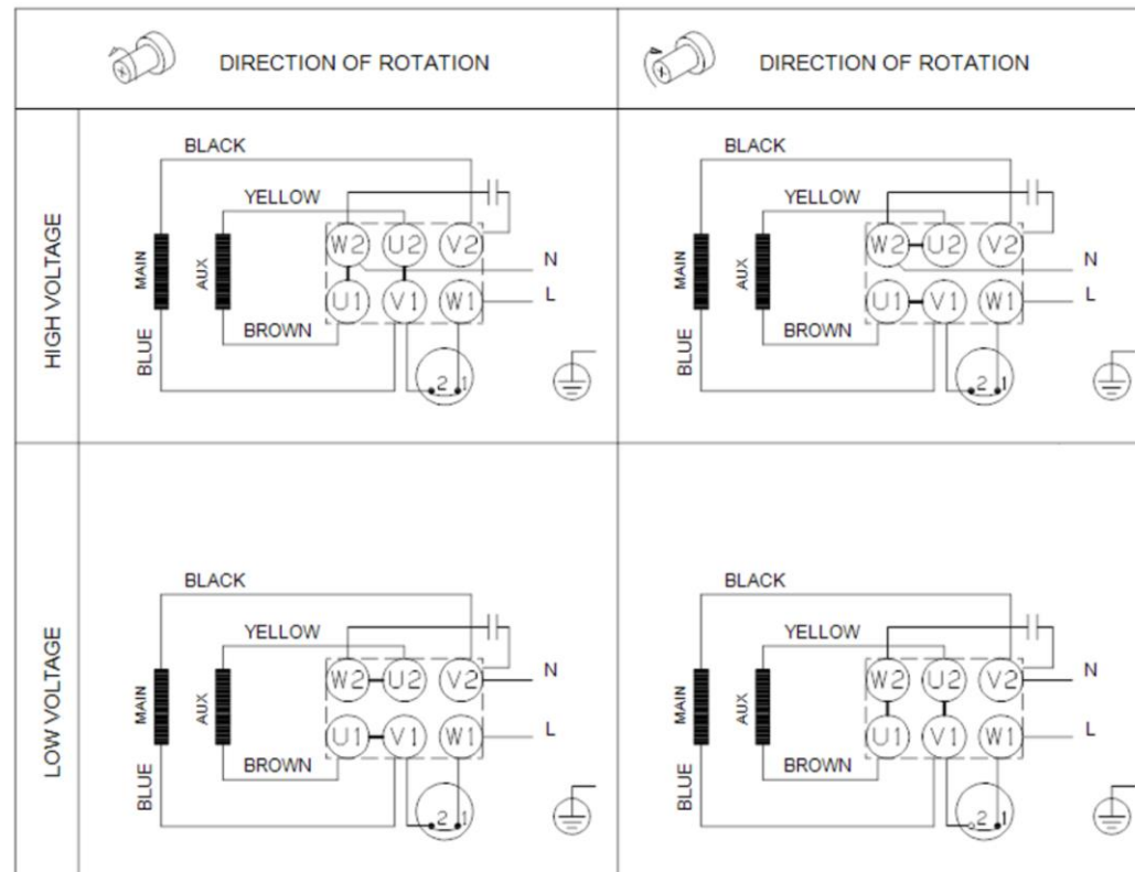
Bomba centrífuga vertical multietapa
