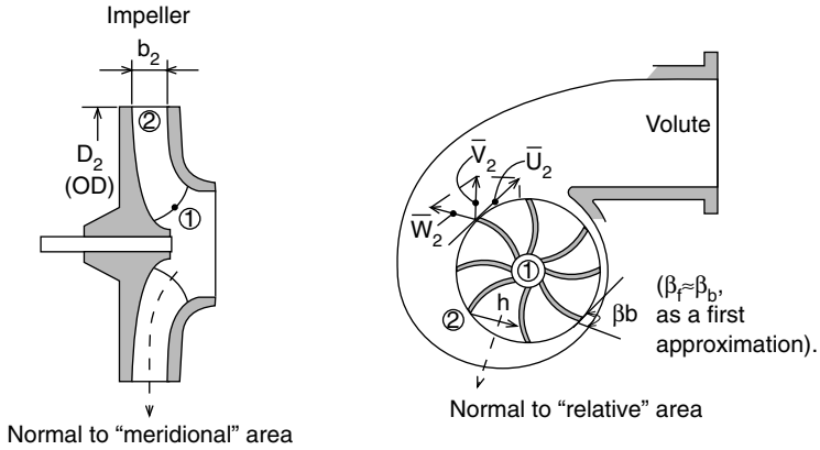
FIGURE 10A A_{m_2} = \pi D_2 b_2 , A_x = b_2 h z z = number of blades (8 here) \bar{u} = peripheral velocity vector \bar{w} = relative velocity vector \bar{v} = absolute (resultant) velocity vector “1” = inlet, “2” = exit of impeller
