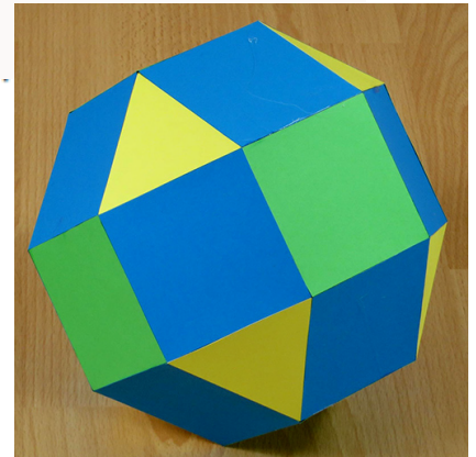
ROMBO-CUBOCTAEDRO
