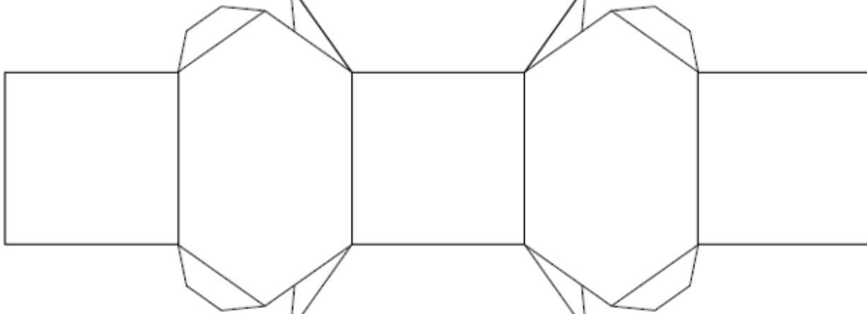
ROMBO-CUBOCTAEDRO
