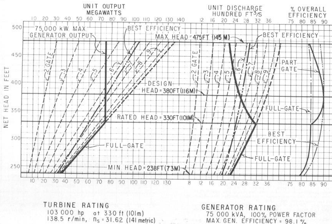
FIGURE 26.—Performance curve—Shasta Powerplant.
