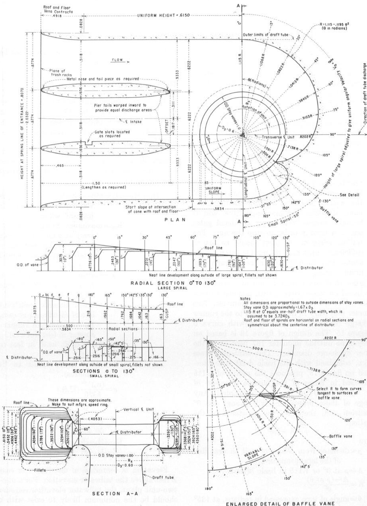
FIGURE 16.—Hydraulic turbine semispiral case—typical proportions.
