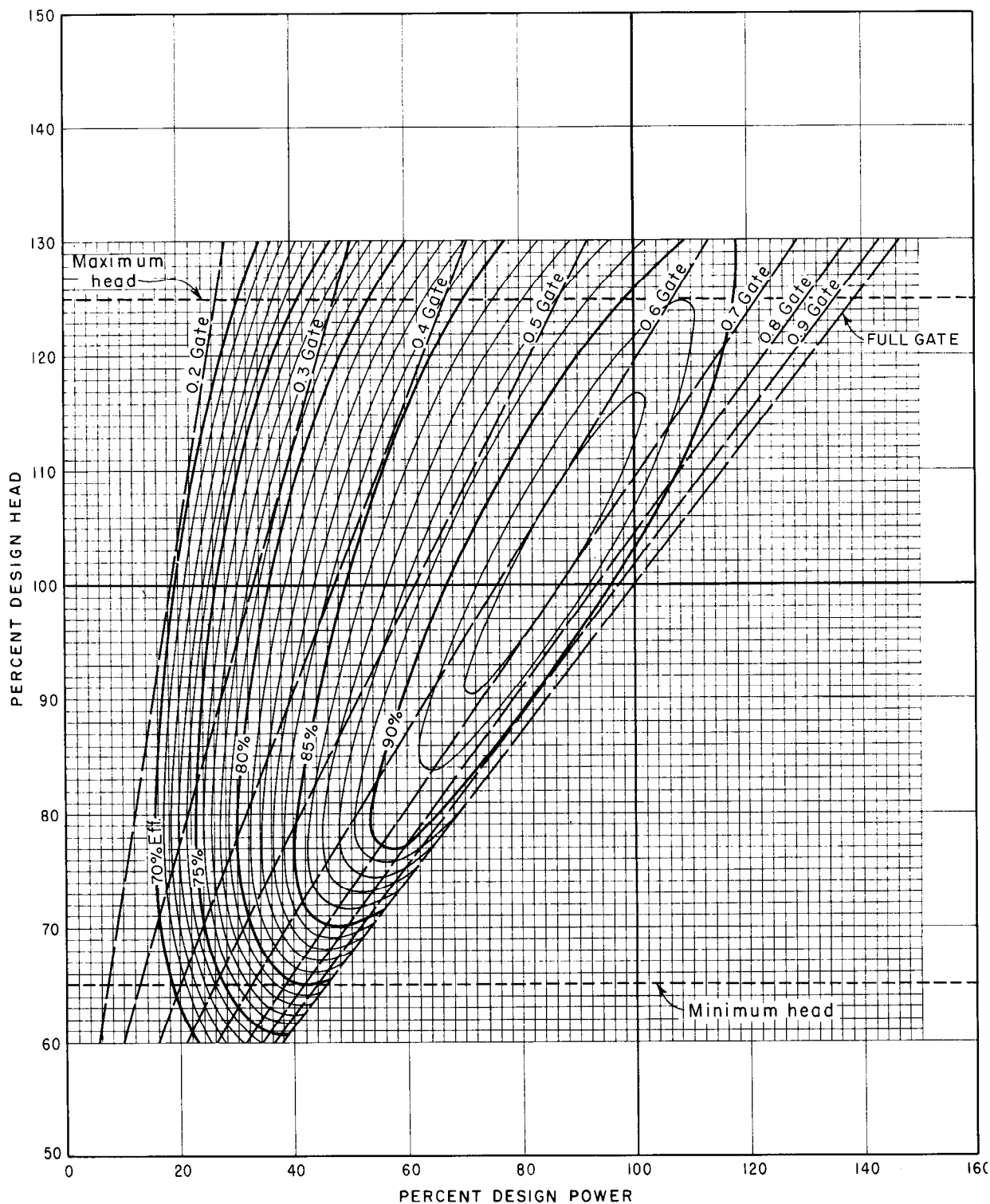
FIGURE 34.—Francis turbine performance—head vs. power— n_s = 40 to 48 (178 to 214 metric).
