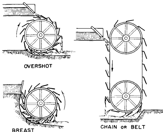
FIGURE 2.—Gravity-type water motors.
