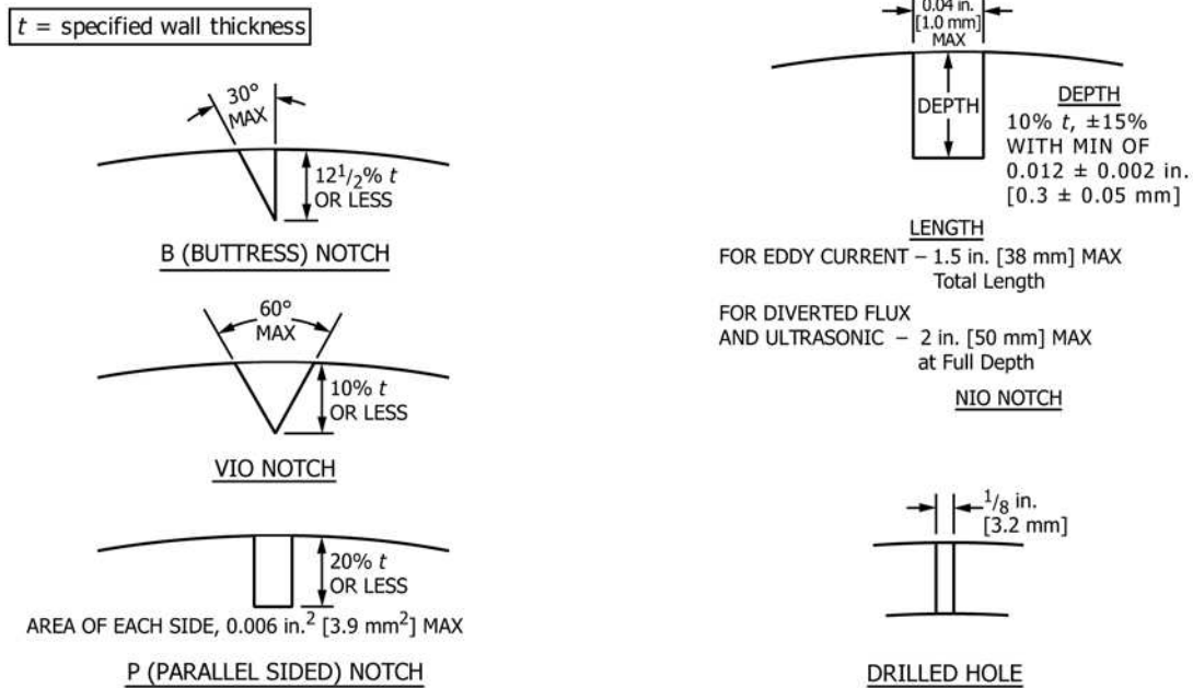
FIG. 1 Calibration Standards
