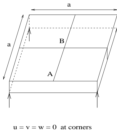
Figure 24. Corner-supported plate ( a = 10 and 1000 , t = 1 , E = 1 \times 10^4 , mesh: 16 \times 16 , \nu = 0.3 , uniform load, q = 1 \times 10^{-8} ).
