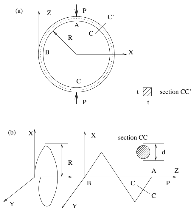
Figure 7. Pinched ring test ( P = 45.45 kg, R = 12.58 cm, t = 0.2388 cm, b = 2.54 cm, E = 0.7398 \times 10^6 kgf/cm 2 , \nu = 0.3125 , \beta^2 = 0.85 , W_A = 3.258 ). Helical spring test ( P = 45.45 kg, R = 25.4 cm, \alpha = 10^\circ , \nu = 0.3 , \beta^2 = 0.886 , d = 2.54 cm, E = 0.71 \times 10^6 kgf/cm 2 , deflection = 7.95 cm).
