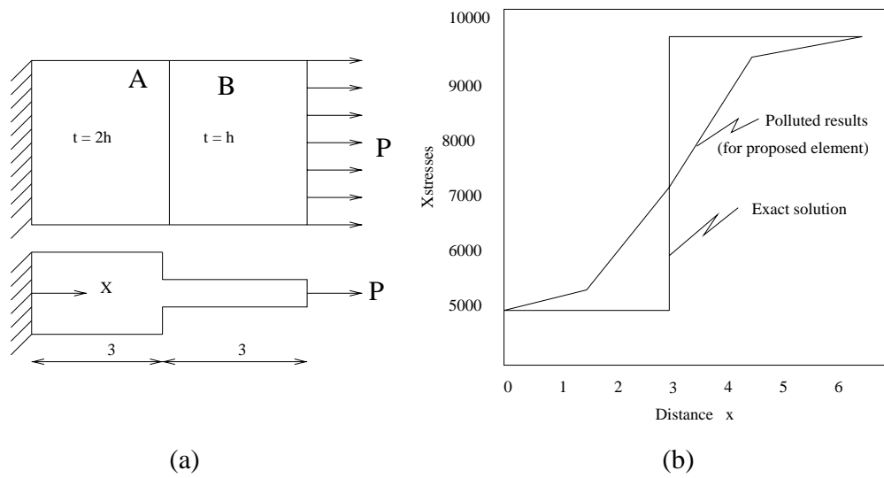
Figure 33. Cantilever beam (stress pollution problem).
