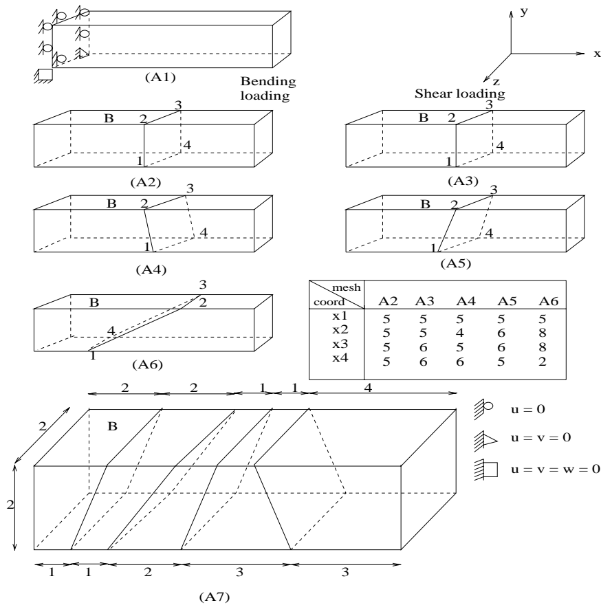
Figure 10. Cheung and Chen tests ( E = 1500, \nu = 0.25, M = 8000, \text{shear} = 600 ).
