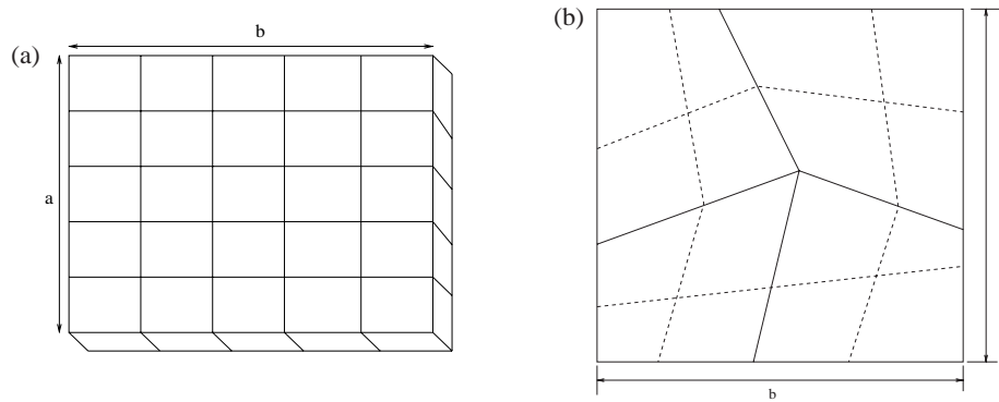
Figure 20. Rectangular plate for convergence and locking tests (a) Mesh: N \times N , a = 2 , b = 2 or 10 , thickness = 0.01 , E = 1.7472 \times 10^7 , \nu = 0.3 , uniform pressure, q = 1 \times 10^{-4} , point load, P = 4 \times 10^{-4} at the plate centre. (b) Distorted mesh.
