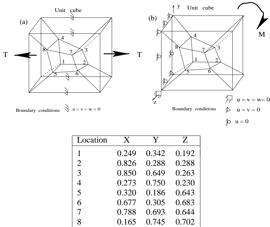
Figure 4. Patch test with three-dimensional warped elements: (a) tension, (b) bending ( E = 1 , tension = 4, M = 4\nu - 0.25 ).
