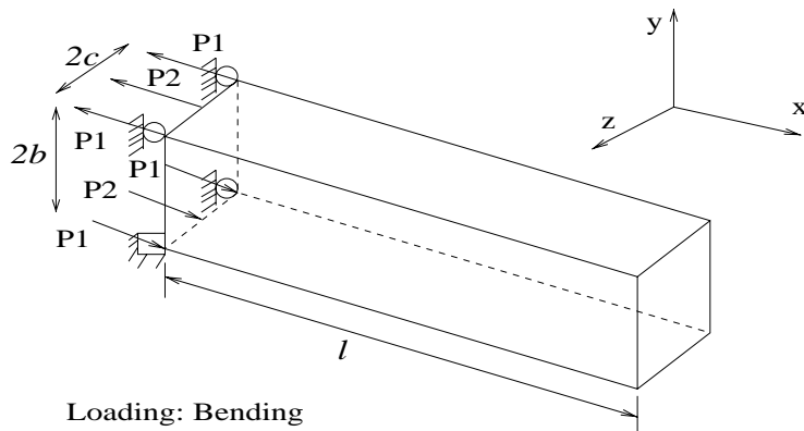
Figure 12. Aspect ratio sensitivity tests ( b = c = 0.06 m, E = 206 \times 10^9 N/m 2 , \nu = 0.25 , M = 1656 N).
