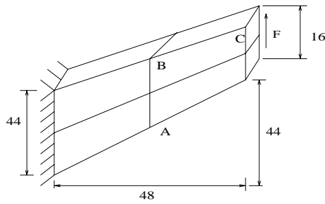
Figure 17. Cook's membrane problem ( E = 1 , thickness = 1, \nu = 0.333 , F = 1 , mesh: 2 \times 2 ).
