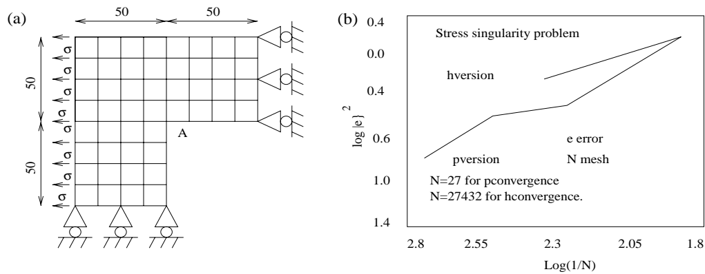
Figure 29. L-shaped domain.
