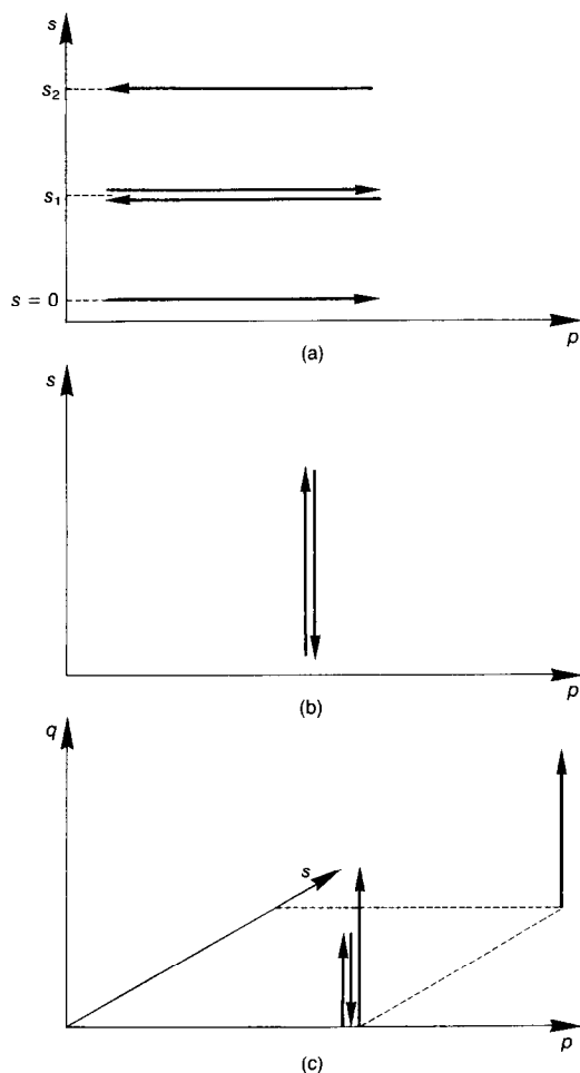
Fig. 9. Suitable stress paths to determine the model parameters
