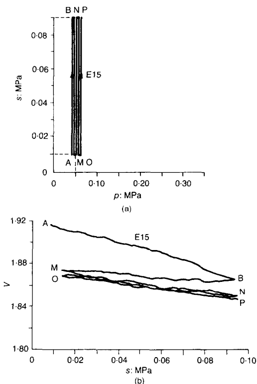
Fig. 18. Effect of cycles of applied suction on changes in specific volume of isotropically confined partially saturated compacted kaolin: (a) stress paths; (b) experimental results
