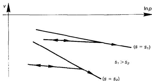
Fig. 1. Proposed variation of specific volume with net mean stress and suction along virgin and unloading-reloading paths
