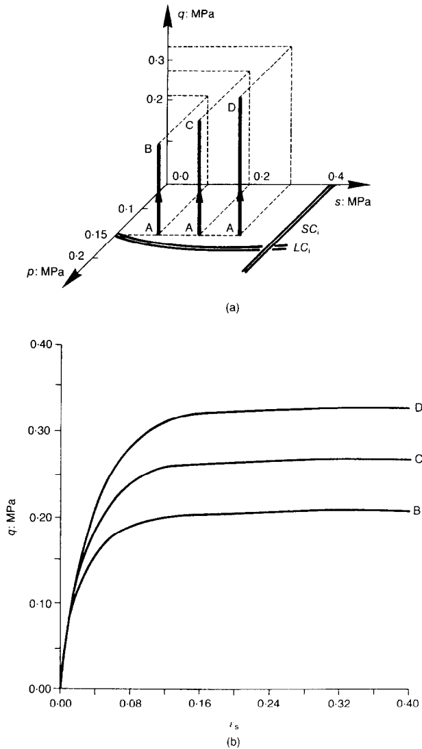
Fig. 15. Response of model to shear tests at different suctions: (a) stress paths; (b) shear stress-shear strain relationships
