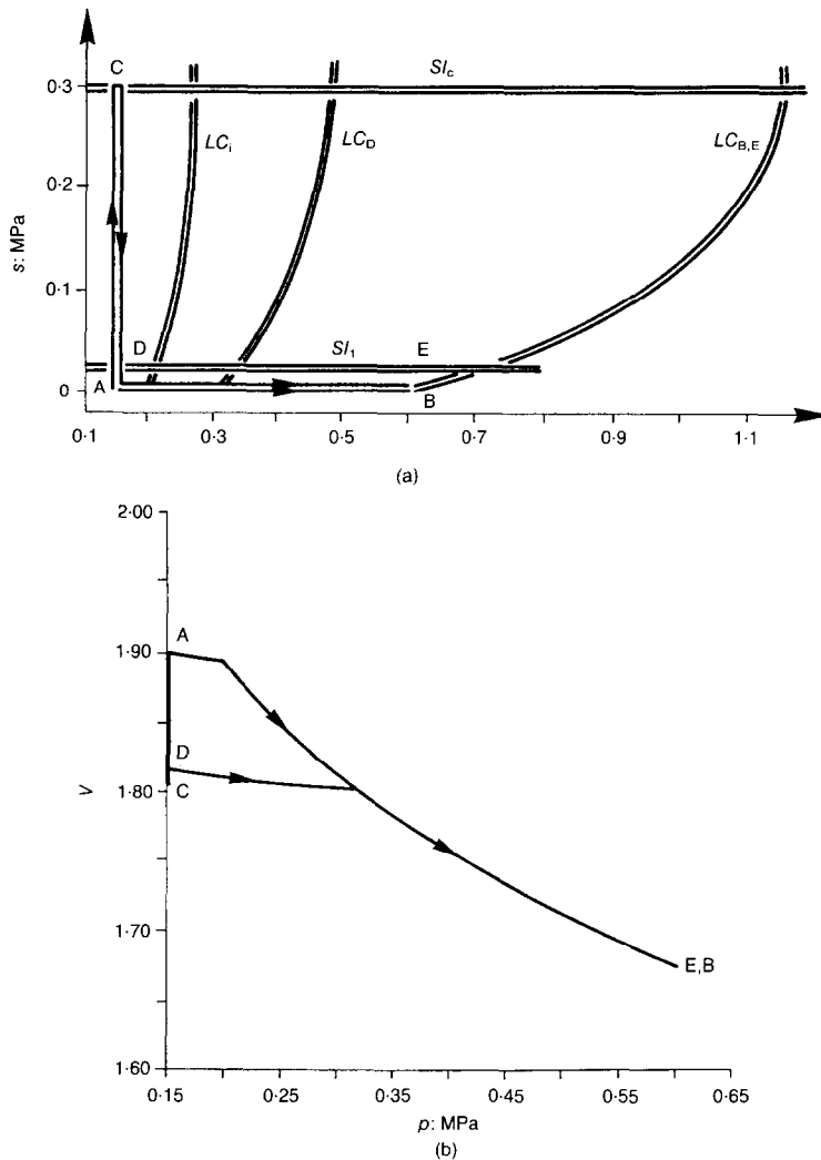
Fig. 14. Effect of initial increase of suction: (a) stress paths; (b) specific volume-net mean stress relationships
