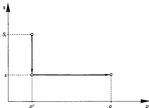
Fig. 3. Wetting and loading stress path in (p, s) stress plane
