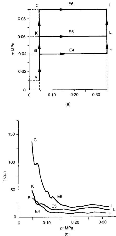
Fig. 17. Isotropic compression tests of partially saturated compacted kaolin: (a) stress paths; (b) variation of soil compressibility
