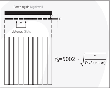
RESONADOR DE HELMHOLTZ A BASE DE LISTONES RESONATOR OF HELMHOLTZ BASED ON SLATS
